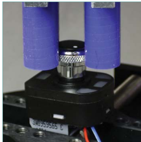
Automotive switch torque test
